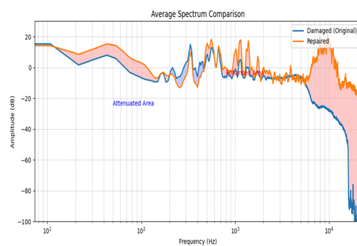
average spectrum comparison (before & after reparation using our model)
