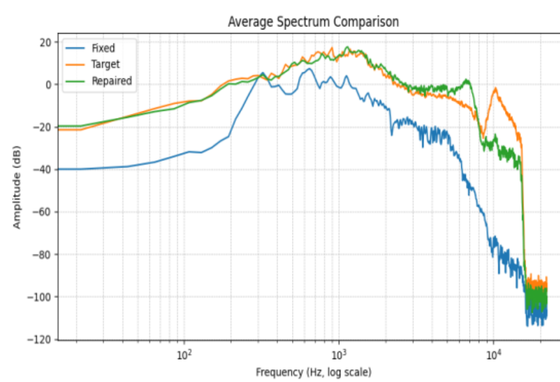
average spectrum comparison (recorded, repaired, original)
